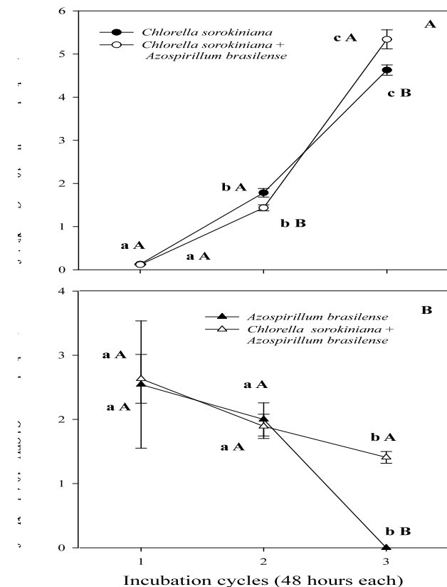
FIG 1. Multiplication of C. sorokiniana (A) and A. brasilense (B) inside of the alginate beads. Points on each curve denoted by a different lower case letter differ significantly at P \leq 0.05 in one way ANOVA. Points denoted by different capital letters after each day of incubation differ significantly P \leq 0.05 at in Student's t -test.
