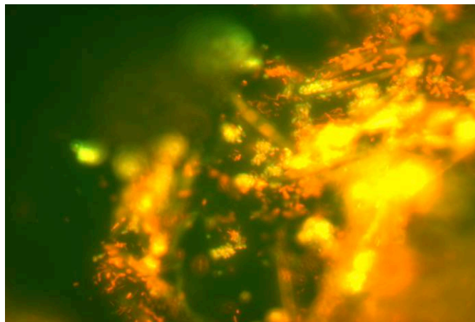
FIG. 2 View of the exterior of the bead. Organism in red are bacteria, organism in yellow are Azospirillum
