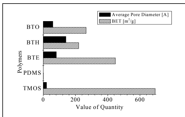
Fig. 1. Polymers porosity characterisation.
