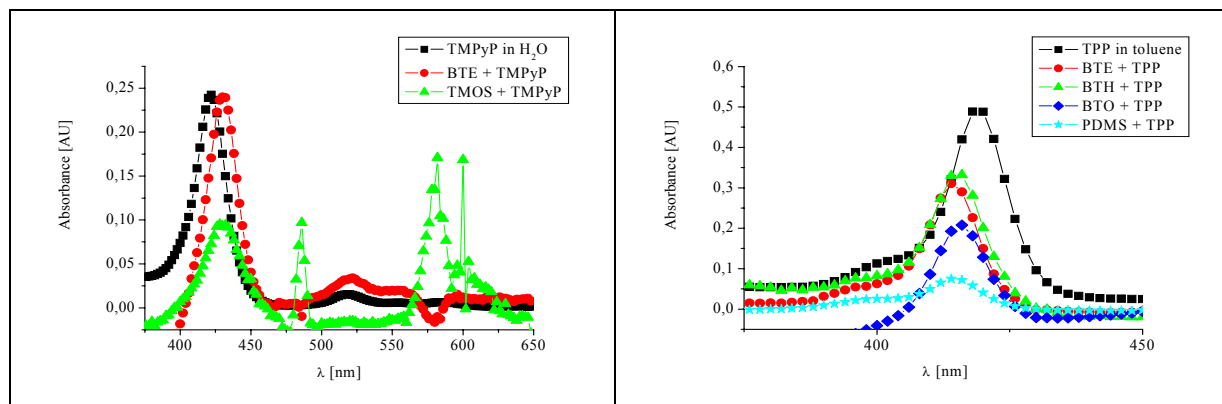
Fig. 2. Spectra of porphyrin-polymer layers and TMPyP solution in deionized water and toluene solution of TPP.
