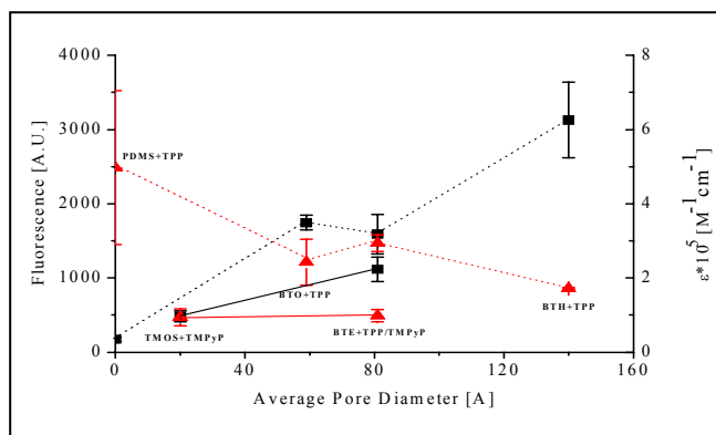
Fig. 3. Intensity of fluorescence and extinction coefficient as a function of pore diameter for polymer-porphyrin layers (■ fluorescence, ▲ \epsilon , — hydrophilic layers, ... hydrophobic layers).
